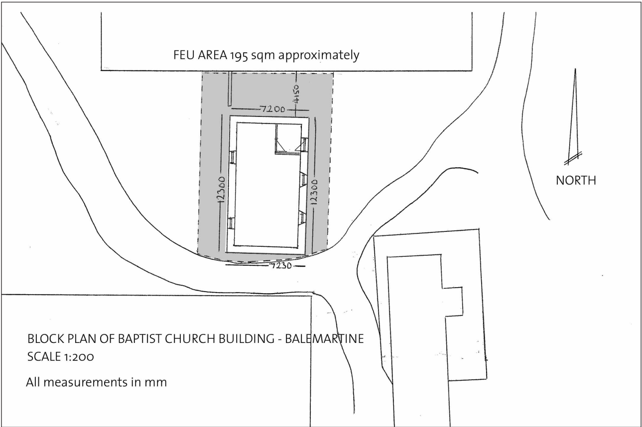
Site Plan
